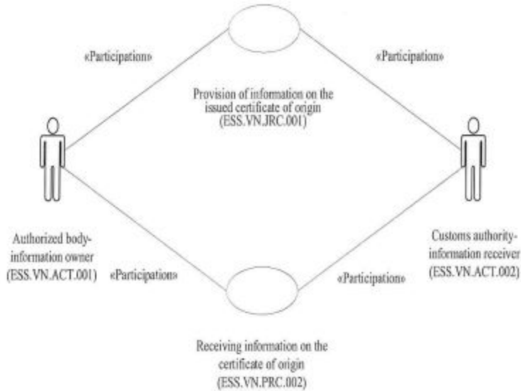
Figure 1. Business process structure
