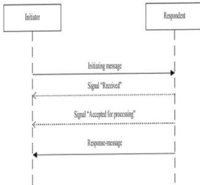
Figure 6. The order of transaction
